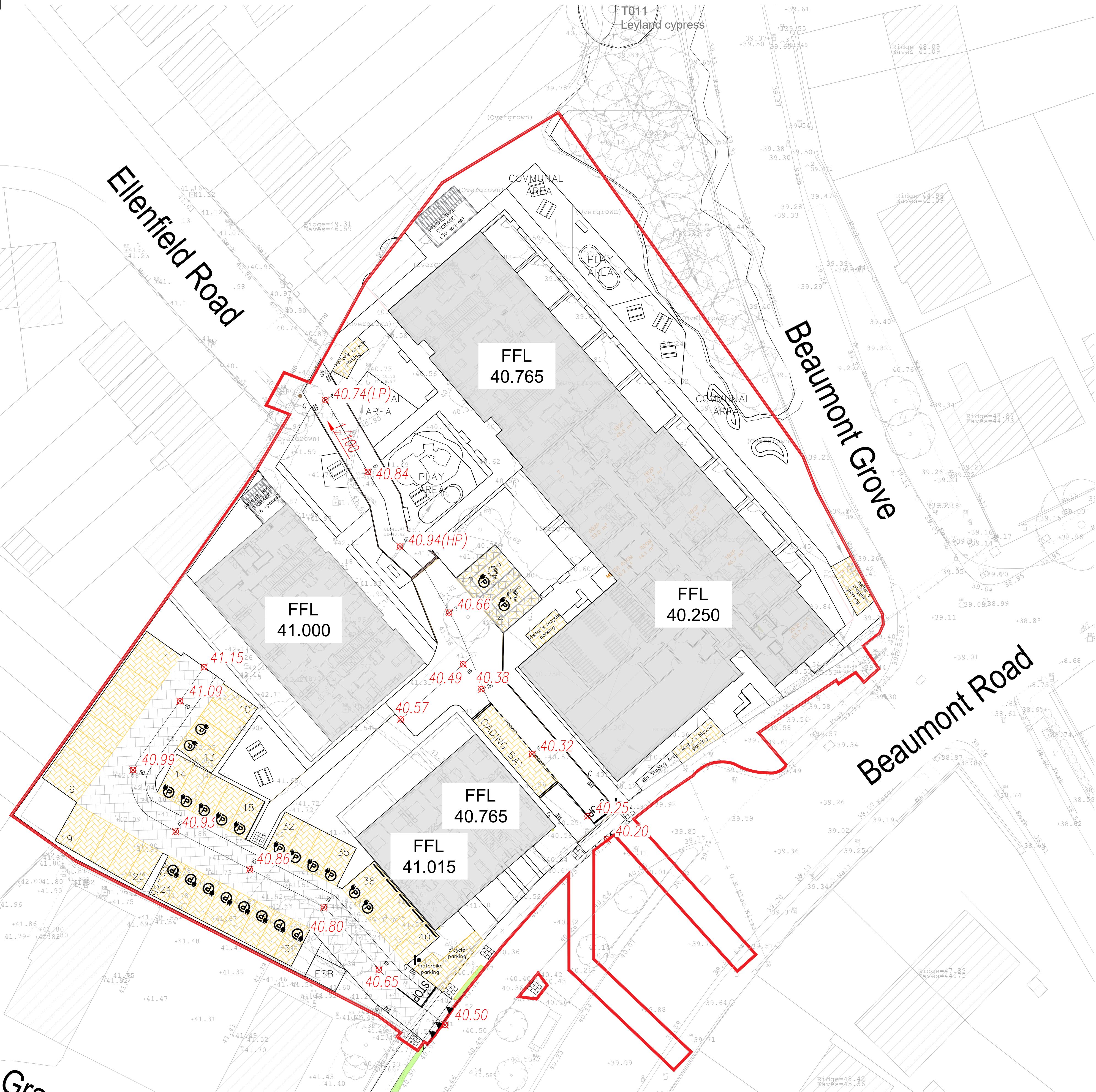
PROPOSED ROAD LAYOUT & LEVELS SCALE 1: 250 @A1
